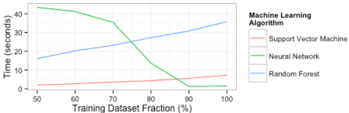
Figure 6: Overall average evaluation speed by training dataset fraction for ORML
